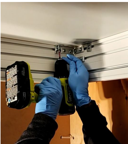
FRAME ASSEMBLY AND ATTACHMENT (COOLEDGE)
